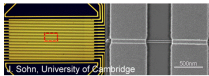
A memory device built around a single zinc oxide nanowire. Each nanowire is less than 100 nm in diameter.
